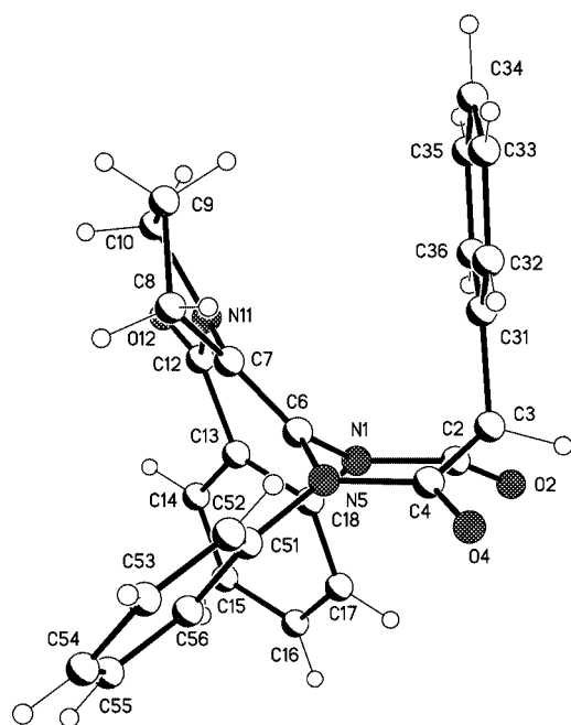
Figure 4. X-ray analysis of 14 . In the single crystal, the dioxopyrimidine fragment of 14 adopts a boat-like conformation with the phenyl ring at C3 in axial position.
