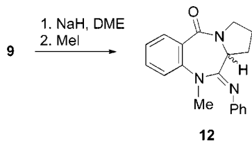
Scheme 5. Methylation of 9 occurs at N(10).
