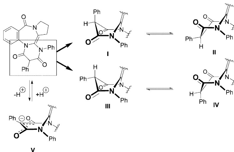
Scheme 7. Boat-chair isomerizations I/II and III/IV (above), and racemizations via anionic species V (below) of the dioxopyrimidine moiety of 14 .
