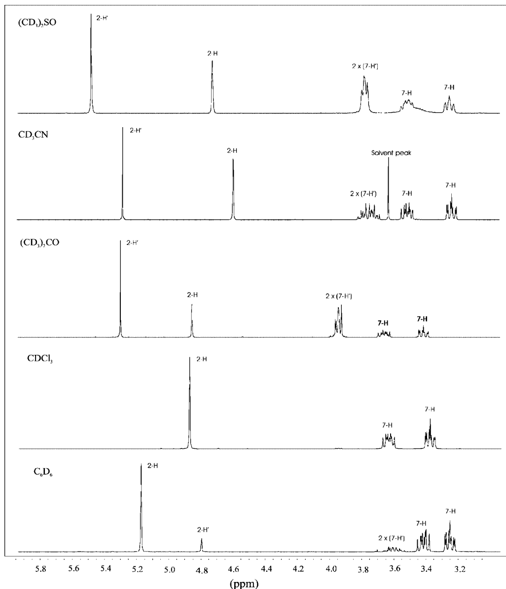
Figure 2. NMR spectra of 14 in various solvents.
