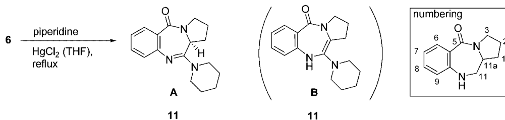
Scheme 4. Tautomeric forms of 11-amino-substituted pyrrolobenzodiazepines.
