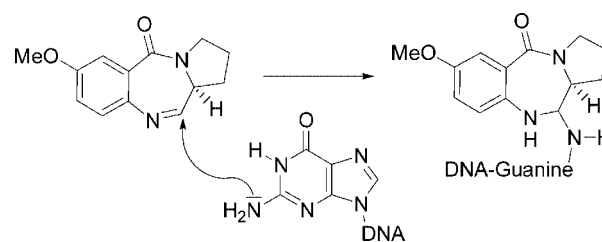
Scheme 1. Attack of guanine on pyrrolobenzodiazepines after insertion into the minor groove of DNA.
