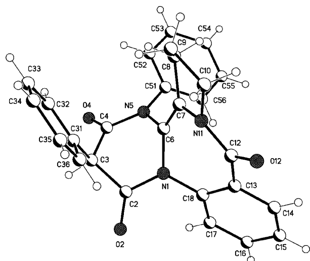
Figure 3. Results of an X-ray analysis of 14 . The drawing shows the helicity of the benzopyrrolodiazepine moiety of 14 .
