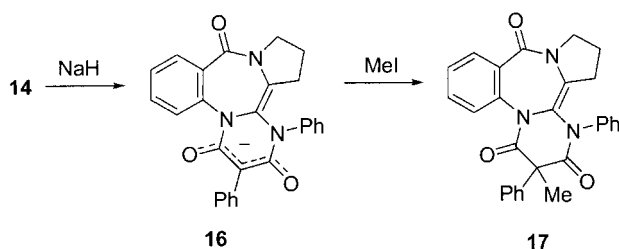
Scheme 8. Deprotonation and methylation.
