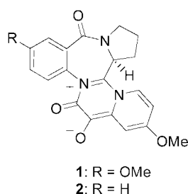
Scheme 2. Proposed structures for circumdatin A ( 1 ) and (B) 2 .
