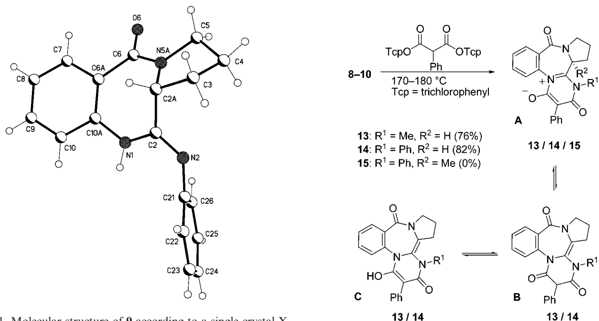
Figure 1. Molecular structure of 9 according to a single-crystal X-ray analysis.
